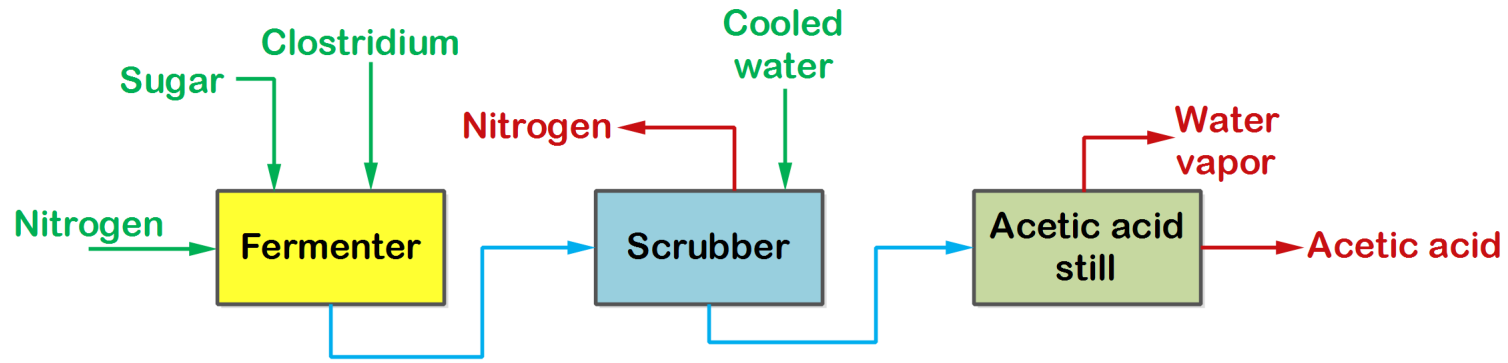
Figure: Manufacture of acetic acid by anaerobic fermentation
